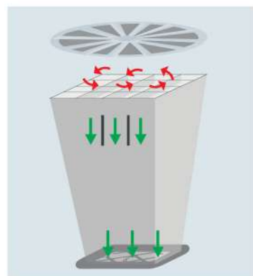
Functional principle of the flow straightener.
